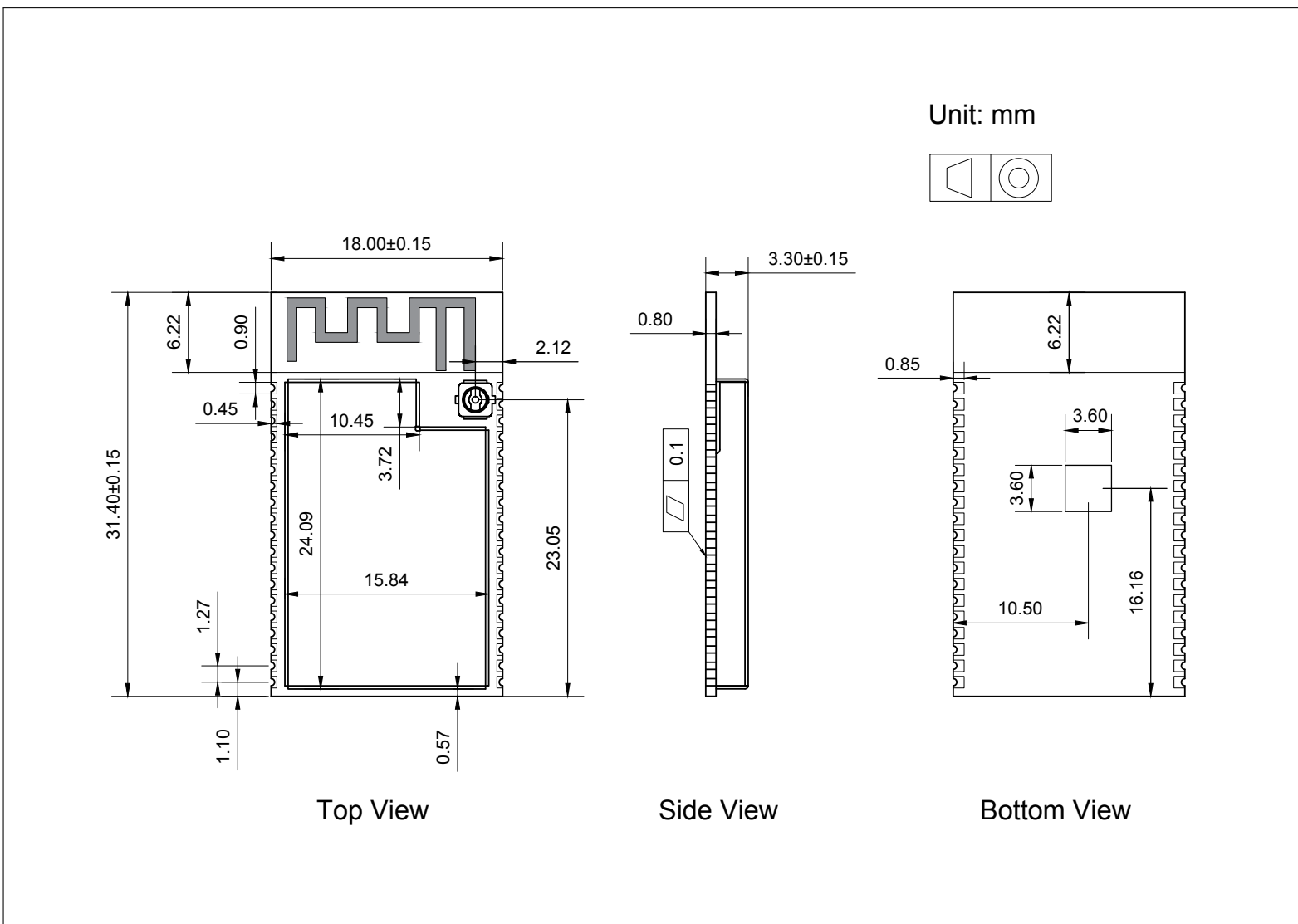
Figure 5: Physical Dimensions of ESP32-WROVER-B (PCB/IPEX)
