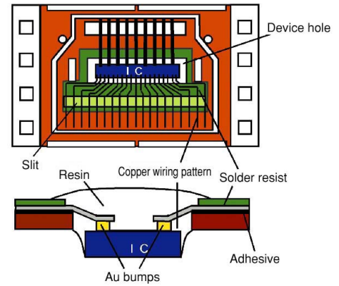
TCP structure
