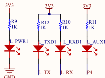
Indicator light
